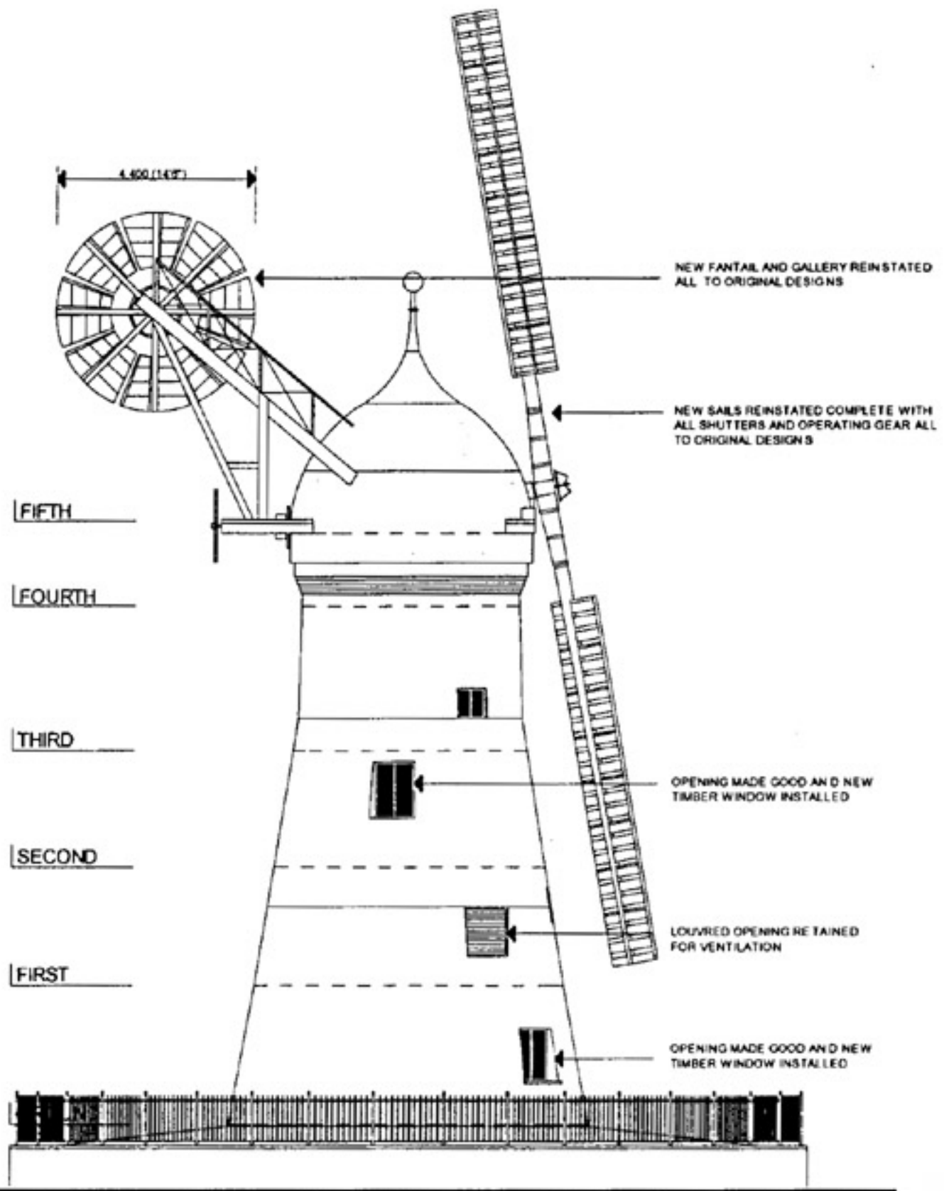
NORTH ELEVATION
