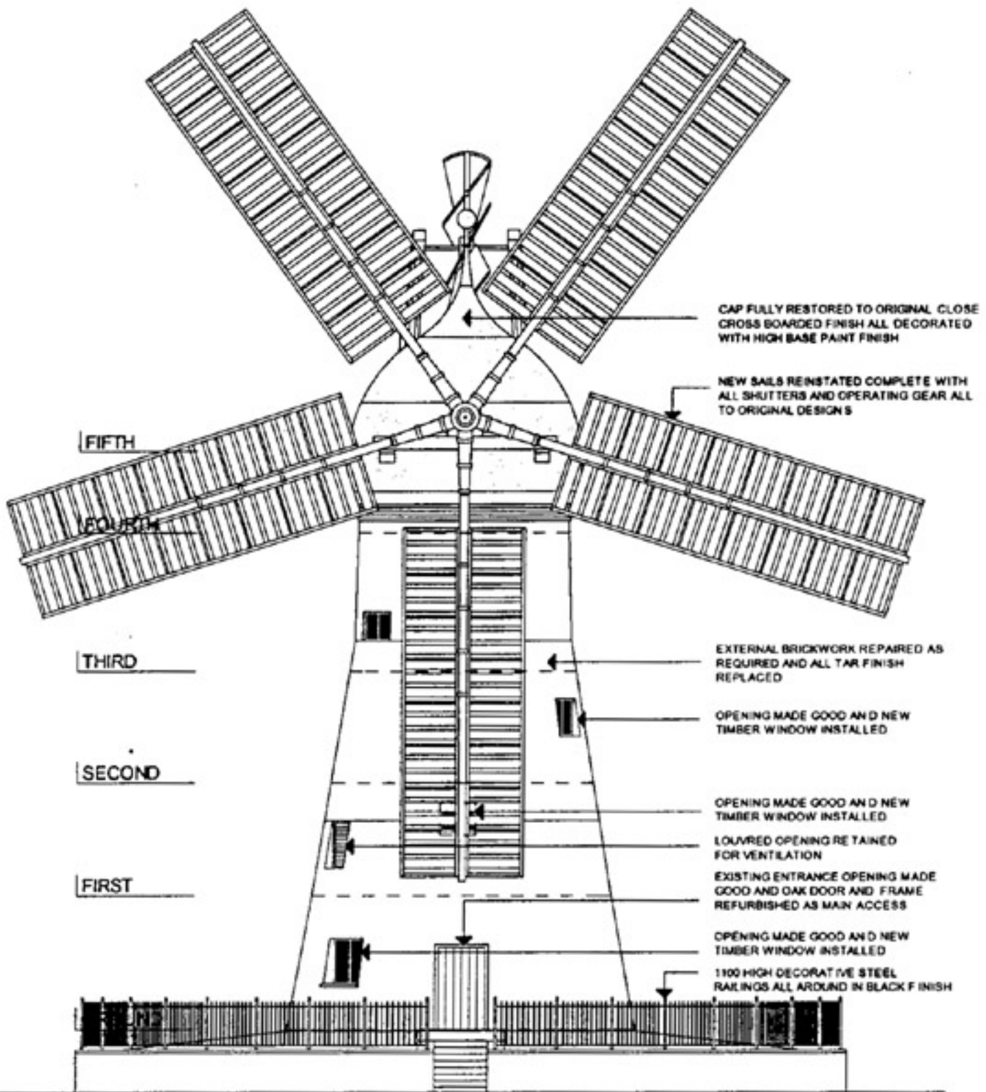
WEST ELEVATION
